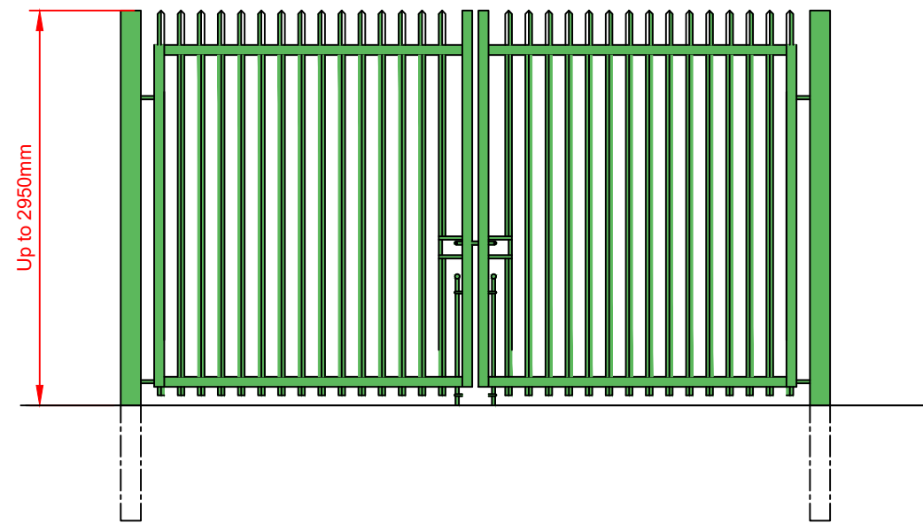
Typical Security Fence Gate Detail (1:50)
