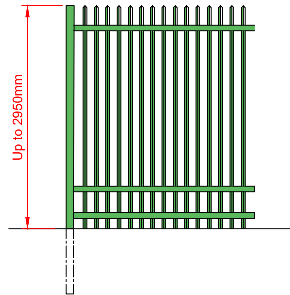
Typical Security Fence Detail (1:50)
